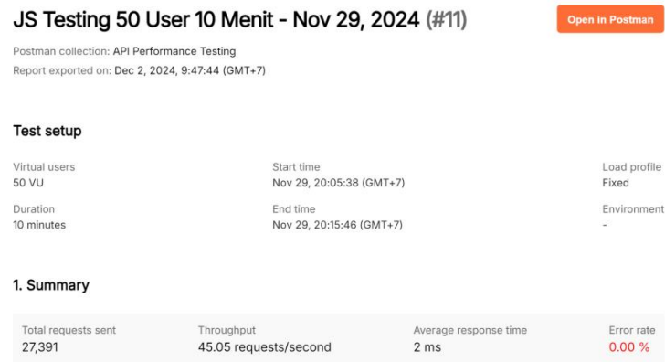
Gambar 5. Report Javascript Testing Fixed 1
