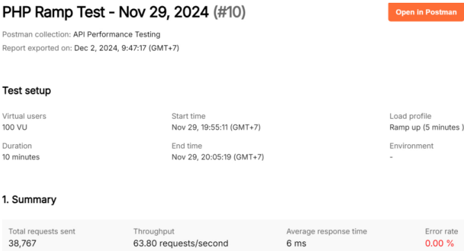
Gambar 11. Report PHP Testing Ramp Up Test
