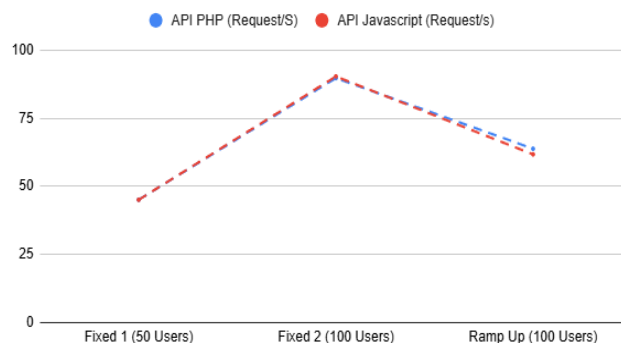
Gambar 16. Grafik Request Per Second
