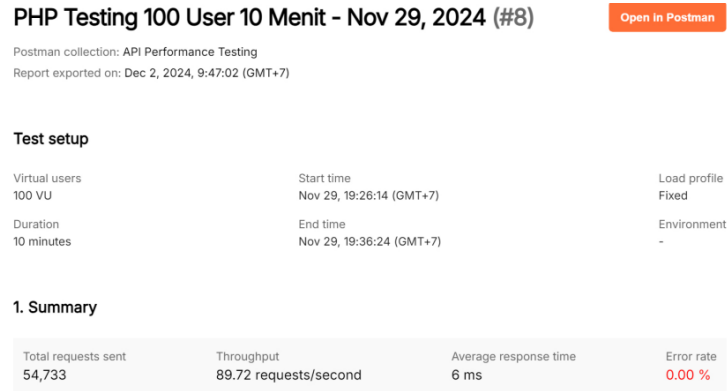
Gambar 7. Report PHP Testing Fixed 2
