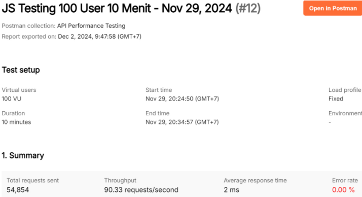
Gambar 9. Report Javascript Testing Fixed 2
