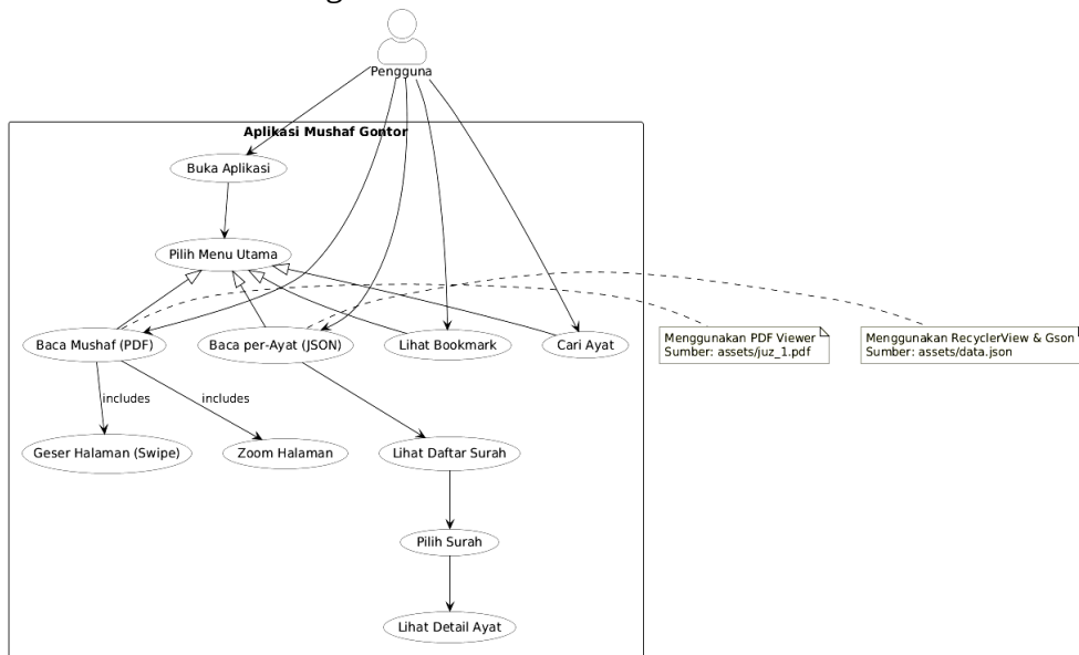
Gambar 1. Usecase Diagram
